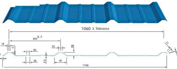
PLANNCO 1060 mm
